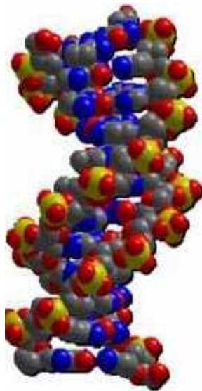
DNA (double helix)
